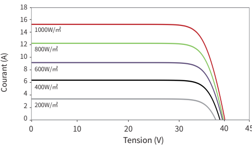
Courbe Courant-Tension (54HL4M-BDV 505W)
